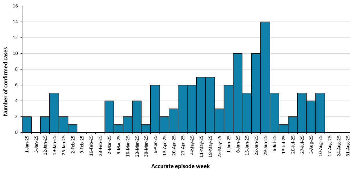
Figure 1: Confirmed Mpox Cases by Week of Accurate Episode Date: Ontario, January 1 to August 31, 2025
