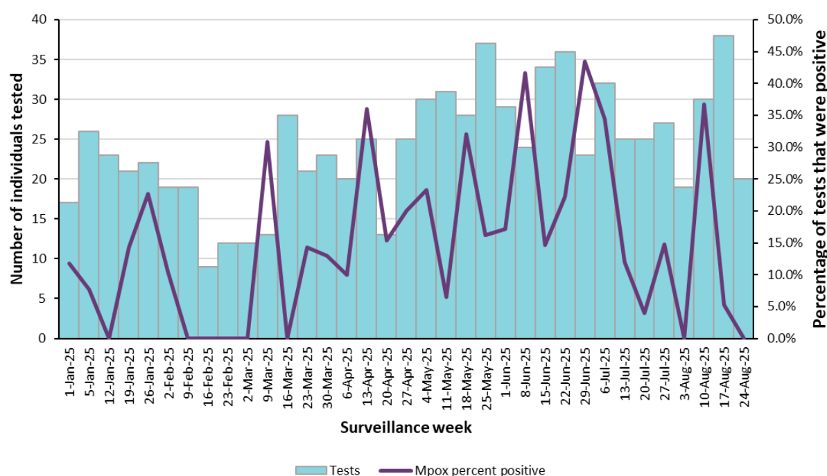
Figure 2: Number of Samples Tested for Mpox and the Number (%) that Tested Positive by Week: Public Health Ontario, January 1 to August 30, 2025
