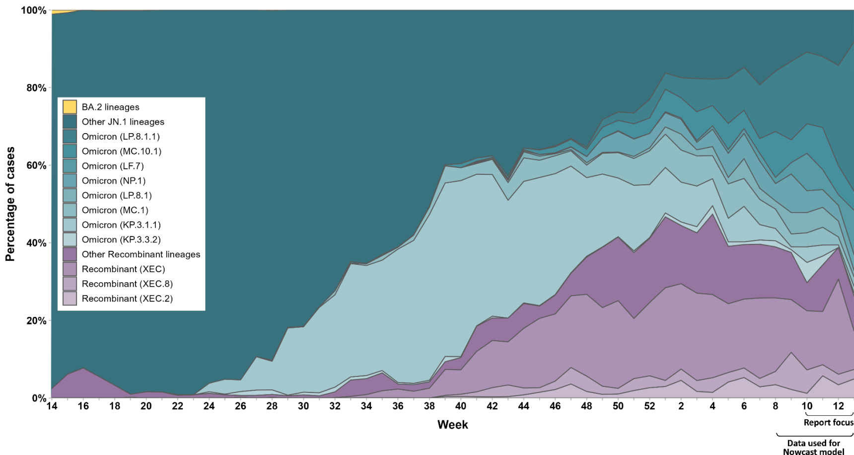
Figure 1: Percentage of SARS-CoV-2 cases by the most prevalent lineages and week, representative surveillance, Ontario, March 31, 2024 to March 29, 2025
