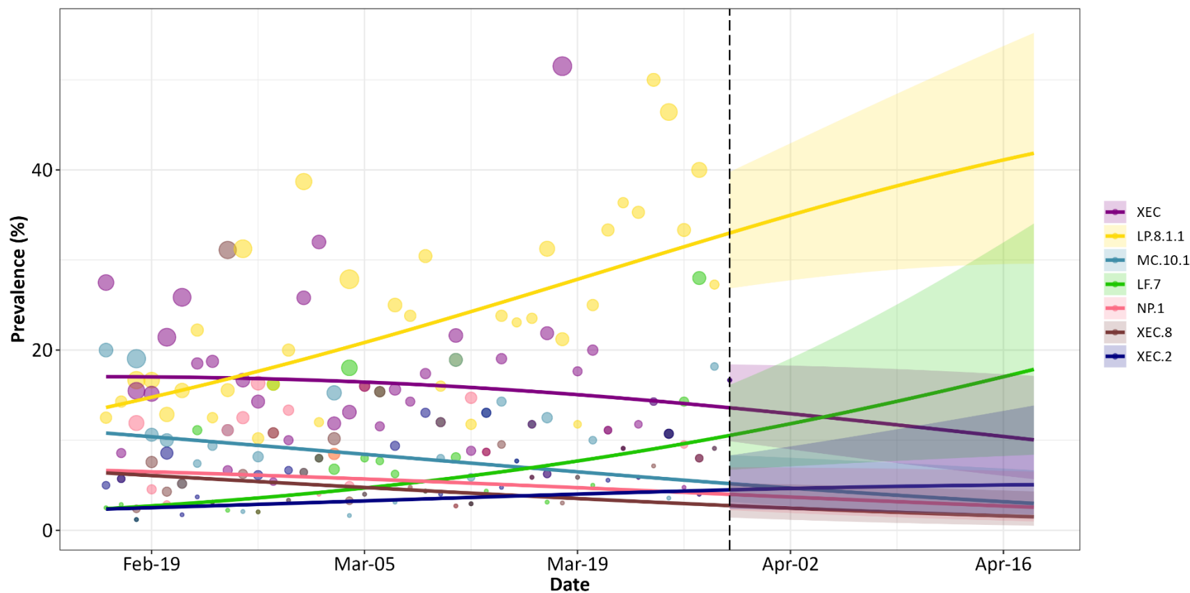
Figure 2: Estimated daily SARS-CoV-2 prevalence (%) by Pango lineage, using Nowcast model, Ontario, February 16 to April 19, 2025
