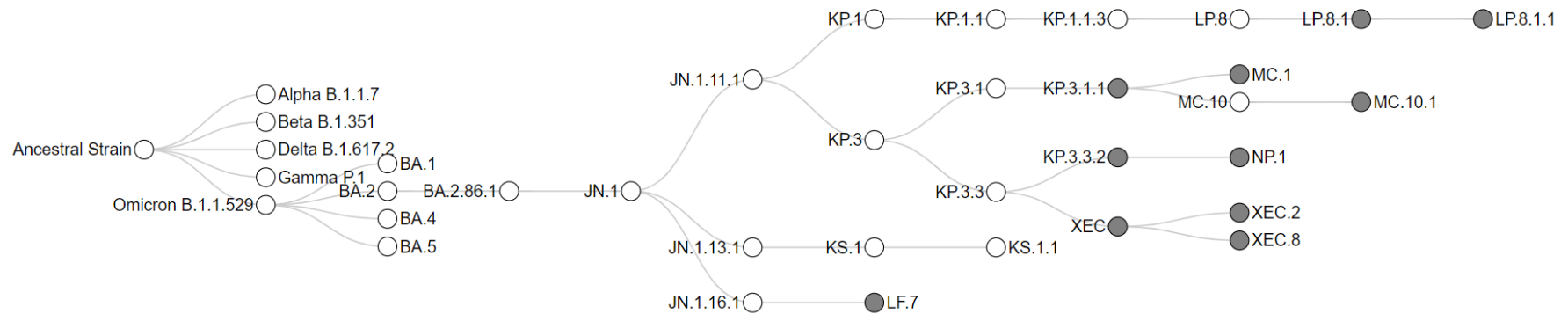
Figure 1: Relationship of the most prevalent SARS-CoV-2 Pango lineages in Ontario, March 2 to March 29, 2025
