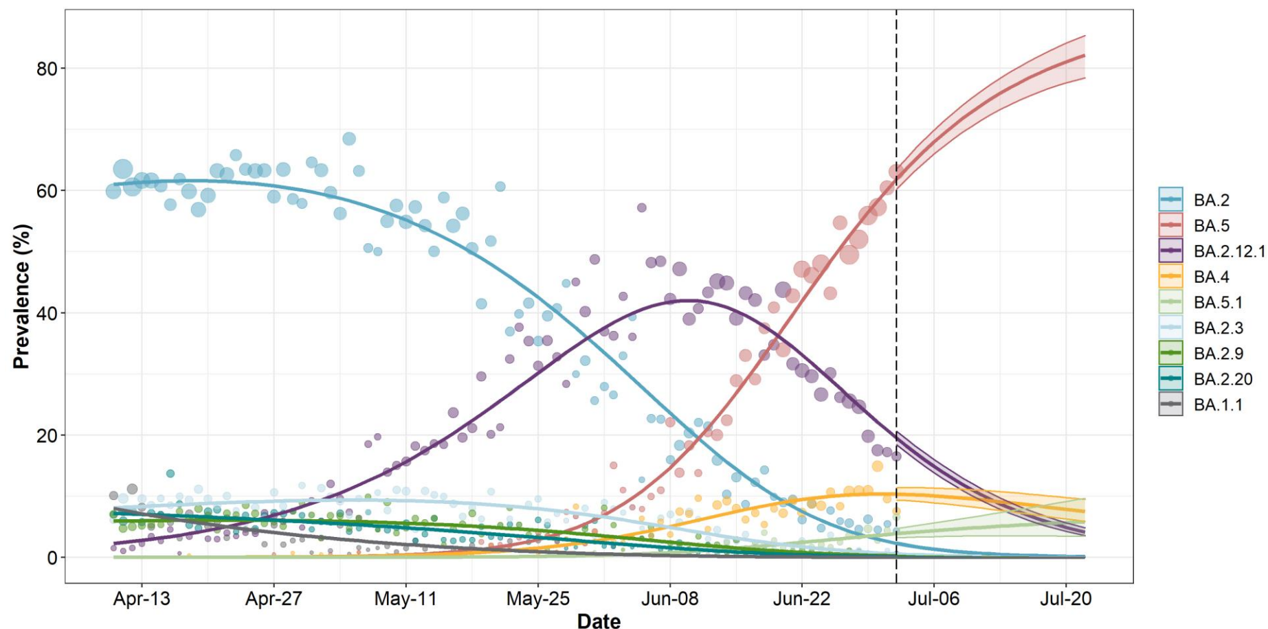
Figure 2. Estimated daily prevalence (%) by Pango lineage, using Nowcast model, Ontario, April 10 to July 23, 2022
