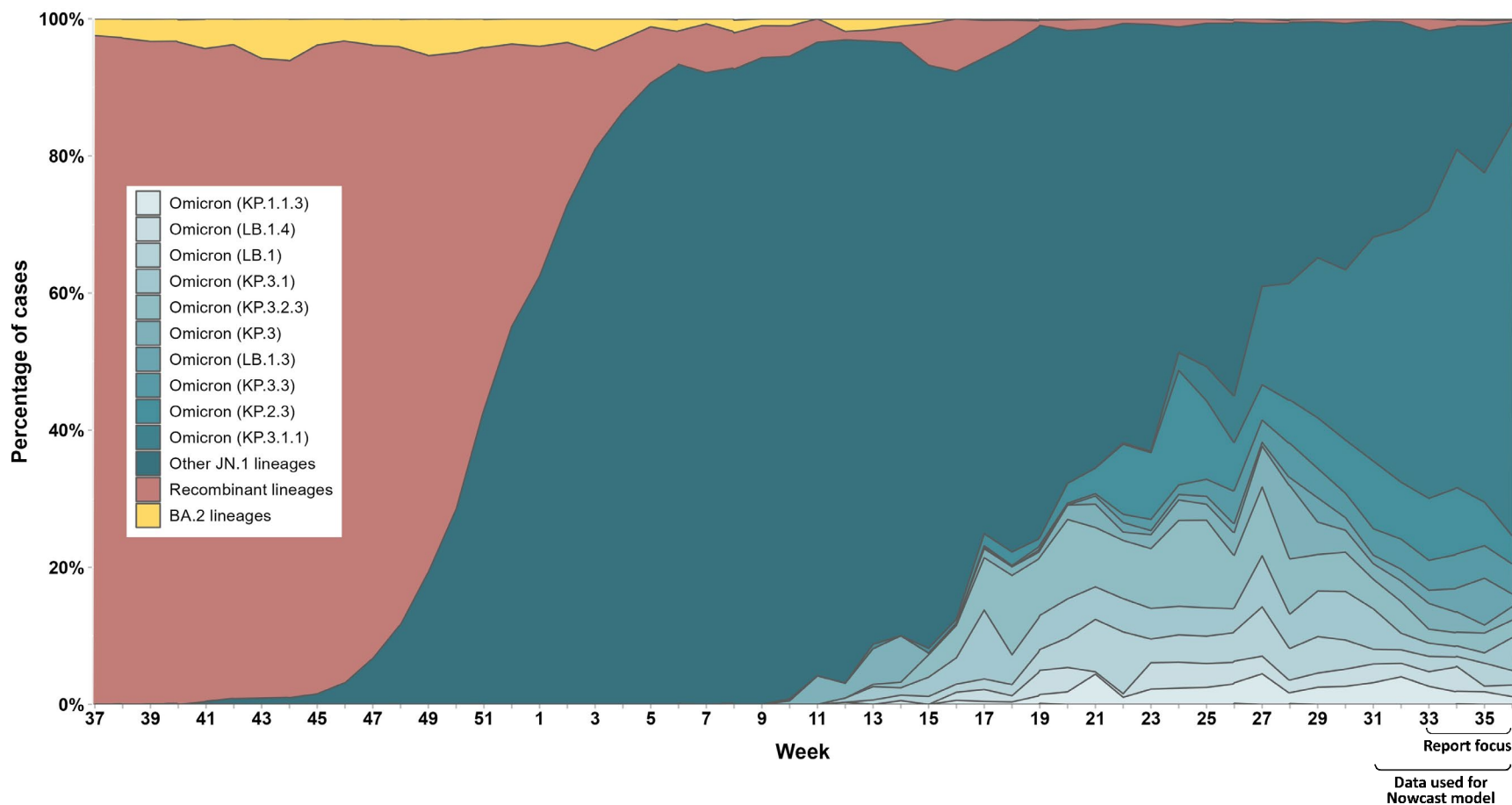
Figure 1. Percentage of SARS-CoV-2 cases by the most prevalent lineages and week, representative surveillance, Ontario, September 10, 2023 to September 7, 2024
