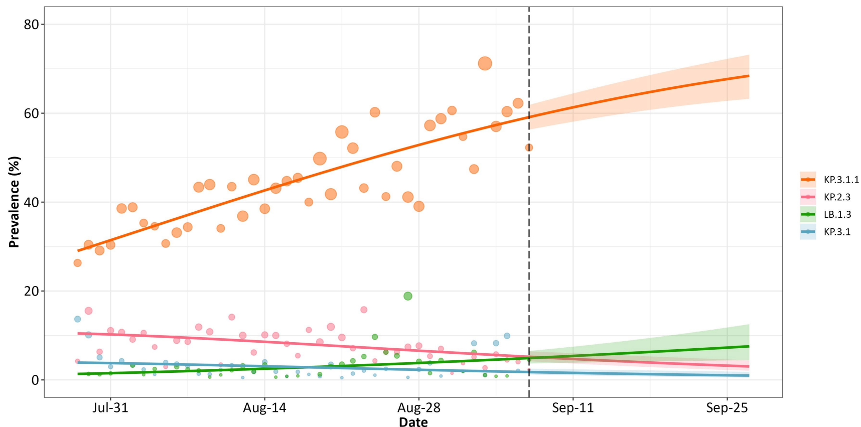
Figure 2. Estimated daily SARS-CoV-2 prevalence (%) by Pango lineage, using Nowcast model, Ontario, July 28 to September 28, 2024
