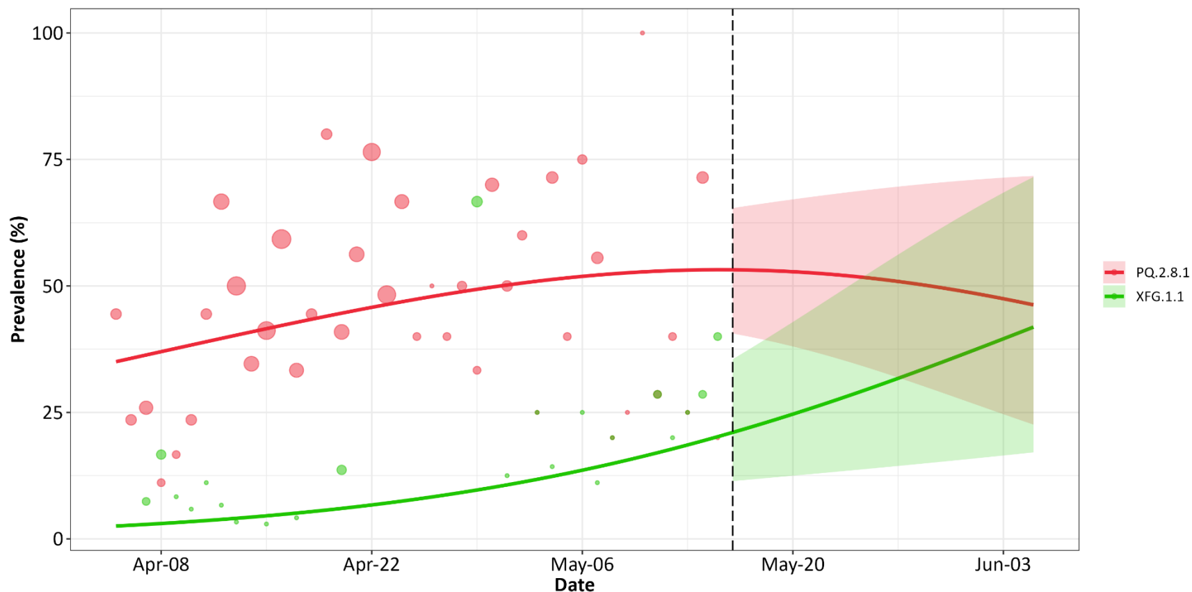
Figure 2: Estimated Daily SARS-CoV-2 Prevalence (%) by Pango Lineage, using Nowcast Model, Ontario, April 5 to June 5, 2026
