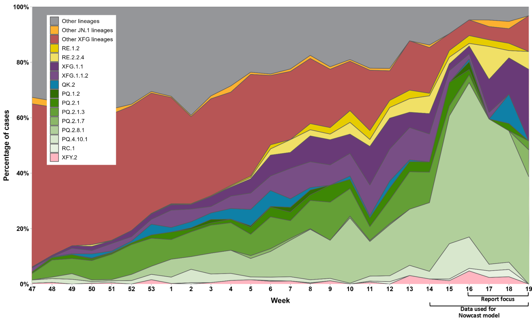
Figure 1: Percentage of SARS-CoV-2 Cases by the Most Prevalent Lineages and Week, Representative Surveillance, Ontario, November 16, 2025 to May 16, 2026
