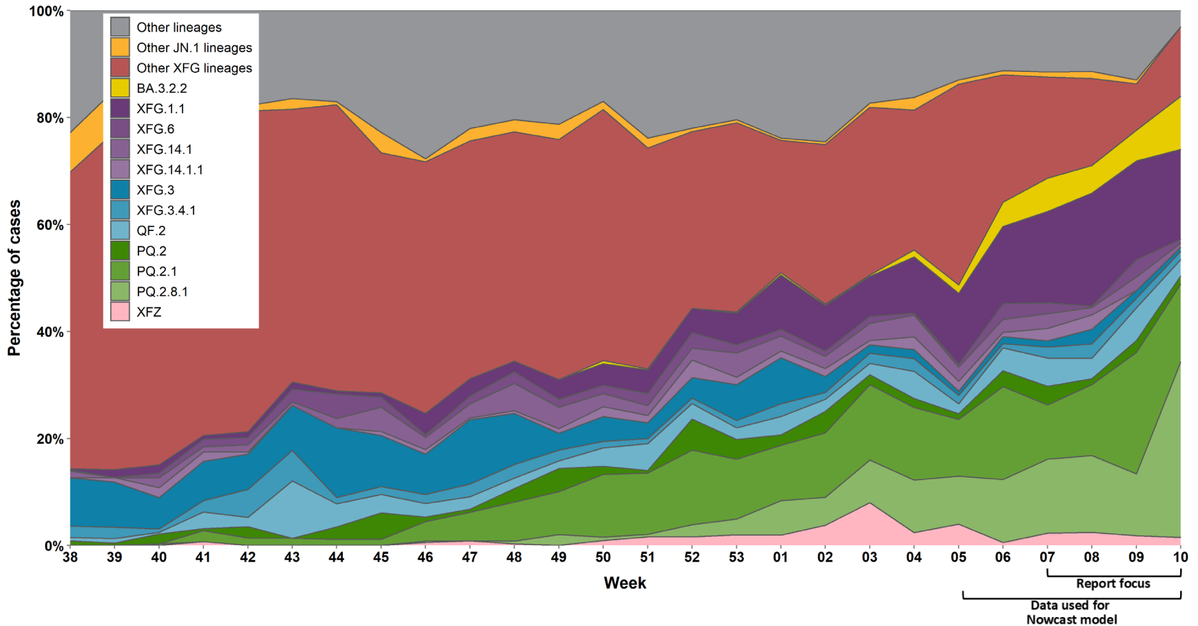
Figure 1: Percentage of SARS-CoV-2 Cases by the Most Prevalent Lineages and Week, Representative Surveillance, Ontario, September 14, 2025 to March 14, 2026
