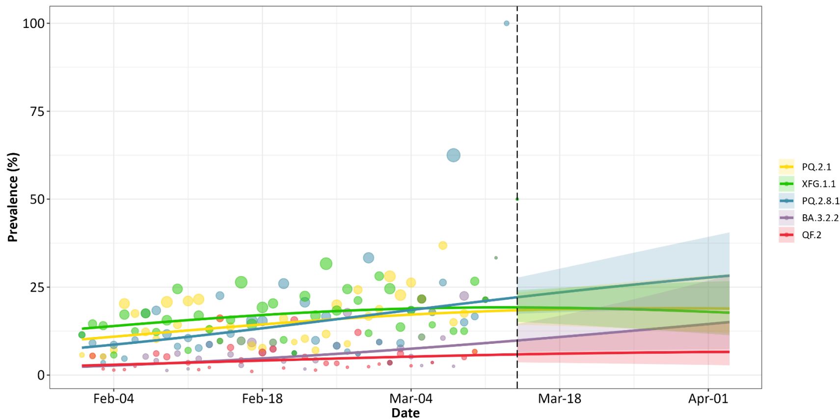
Figure 2: Estimated Daily SARS-CoV-2 Prevalence (%) by Pango Lineage, using Nowcast Model, Ontario, February 1 to April 3, 2026
