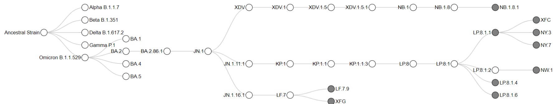
Figure 1: Relationship of the most prevalent SARS-CoV-2 Pango lineages in Ontario, June 22 to July 19, 2025
