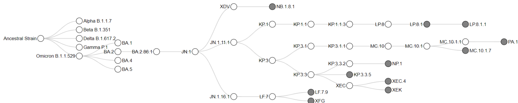
Figure 1: Relationship of the most prevalent SARS-CoV-2 Pango lineages in Ontario, April 20 to May 17, 2025
