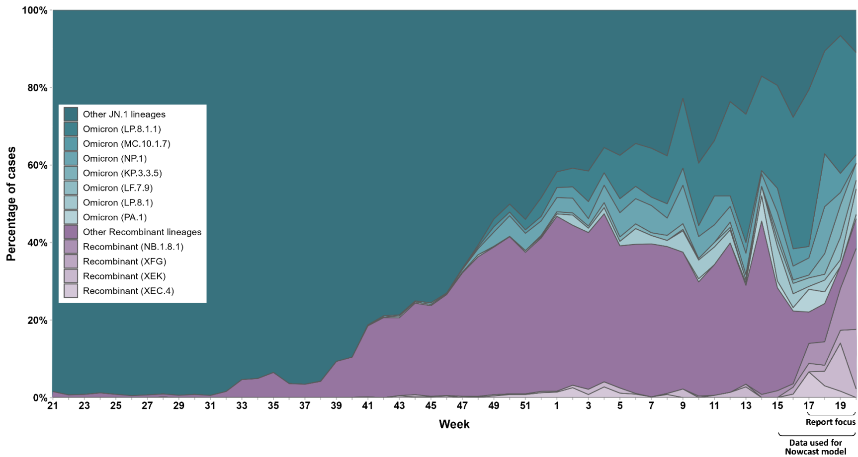
Figure 1: Percentage of SARS-CoV-2 cases by the most prevalent lineages and week, representative surveillance, Ontario, May 19, 2024 to May 17, 2025
