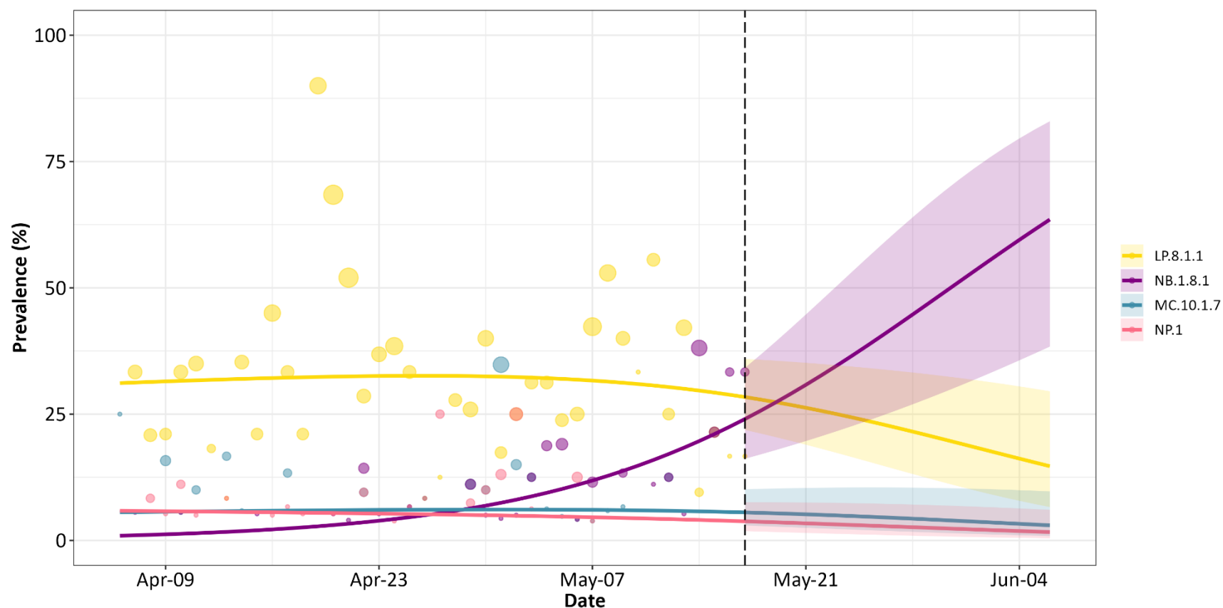
Figure 2: Estimated daily SARS-CoV-2 prevalence (%) by Pango lineage, using Nowcast model, Ontario, April 6 to June 7, 2025
