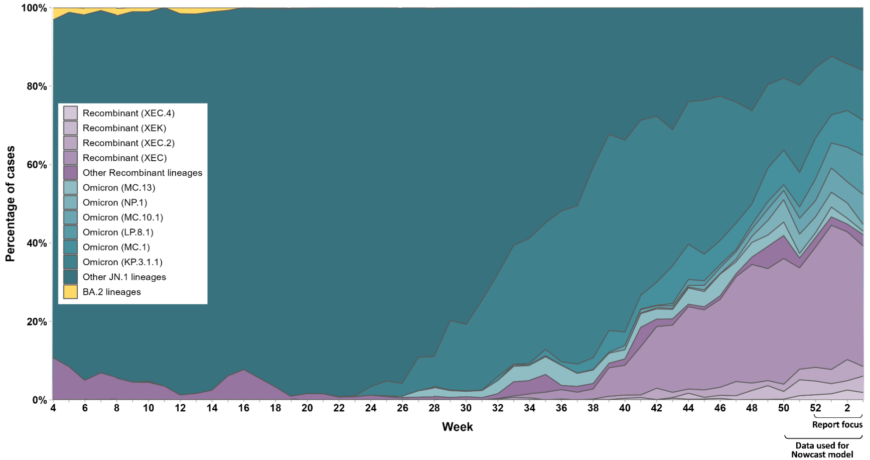
Figure 1: Percentage of SARS-CoV-2 cases by the most prevalent lineages and week, representative surveillance, Ontario, January 21, 2024 to January 18, 2025
