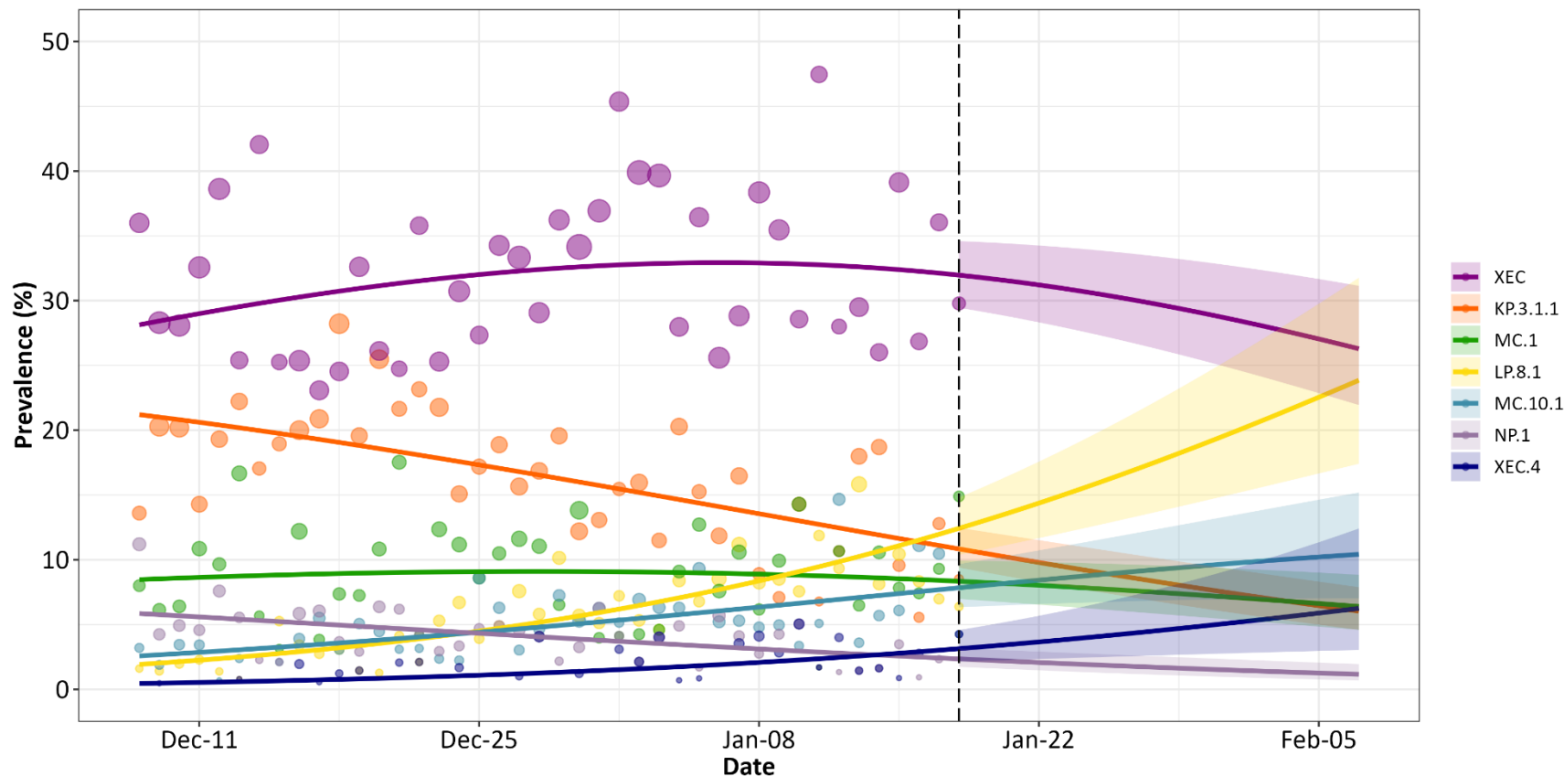
Figure 2: Estimated daily SARS-CoV-2 prevalence (%) by Pango lineage, using Nowcast model, Ontario, December 8, 2024 to February 8, 2025
